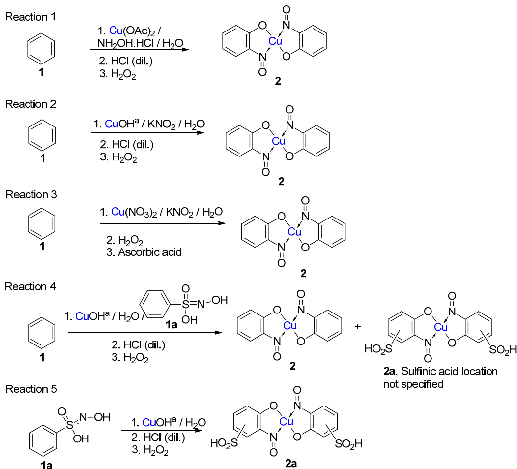
Scheme 1. Five different reactions (1–5) that Baudisch chose to publish, across two publications, which have subsequently become known as the Baudisch reaction [20,21]. *Baudisch states in the literature that ‘freshly prepared yellow cuprous hydroxide’ was used; it is known that this is not a stable entity, so the actual active substance could well be an alternative such as cuprous oxide, \text{Cu}_2\text{O} .
