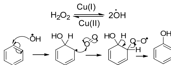
Scheme 8. The mechanism under which phenol is formed from benzene [42,43].
