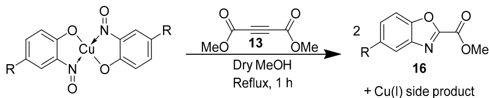
Scheme 11. The general procedure reported for benzoxazole synthesis [75].
