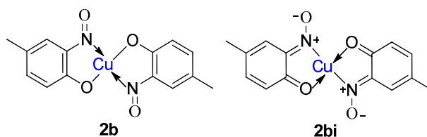
Figure 3. The possible tautomers of copper(II) bis (4-methyl-2-nitrosophenolato), (2b, 2bi).
