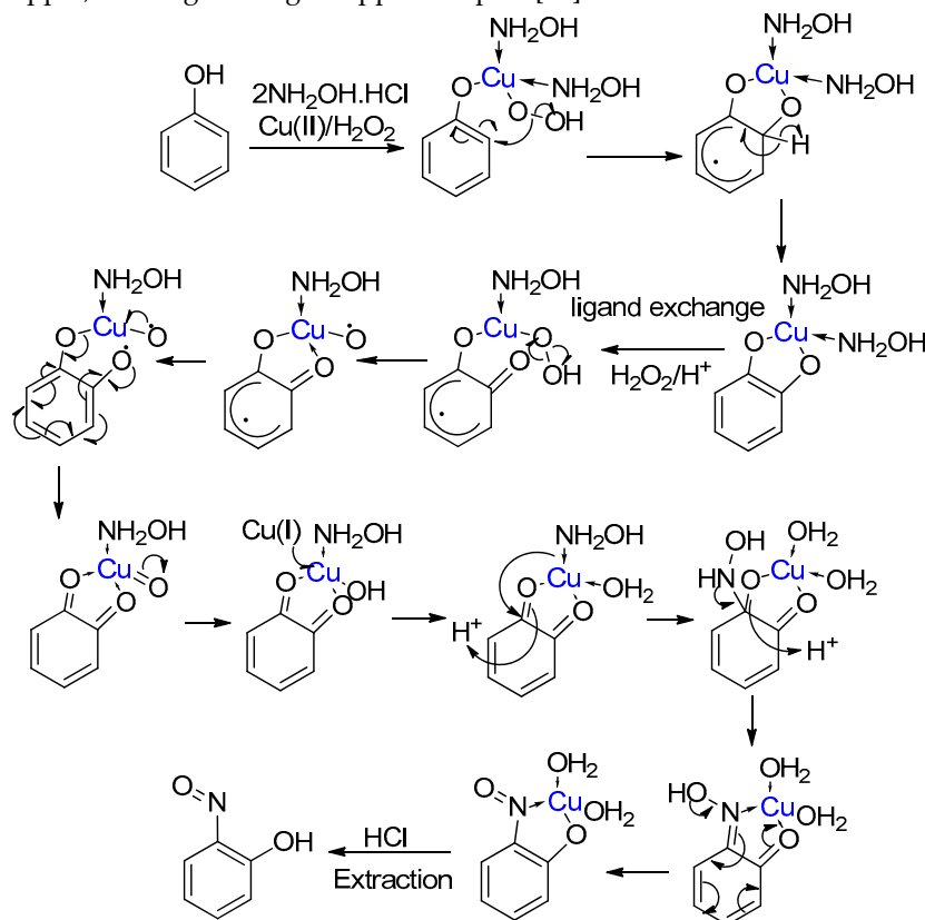
Scheme 9. The accepted mechanism for the Baudisch Reaction with hydroxylamine [26,42].
