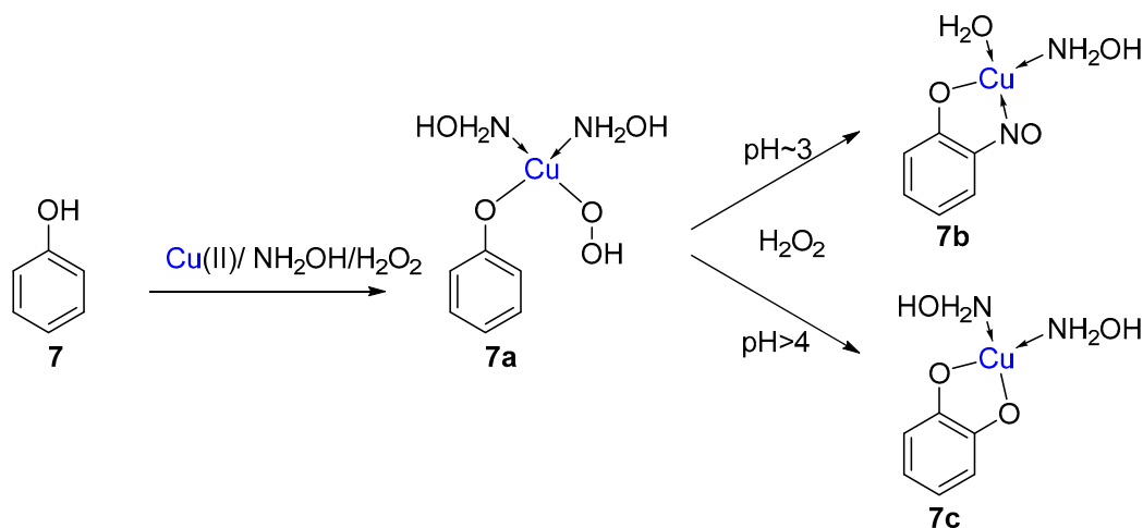
Scheme 5. The suggested common intermediate complex ( 7a ) between the reactions at different pH. At a \text{pH} \sim 3 , the favoured path leads to the copper 2-nitrosophenol complex ( 7b ), while at a \text{pH} > 4 the preferred pathway leads to catechol ( 7c ).
