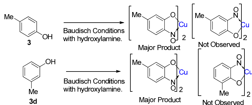
Scheme 10. The results of reactions of methyl-substituted phenols show that the favoured product has the methyl group para to the nitroso (n.b. given of course the nitroso must also be ortho to the phenol).
