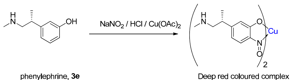
Figure 8. Dessouky's colourimetry determination of phenylephrine, an example of copper-mediated nitrosation [25].
