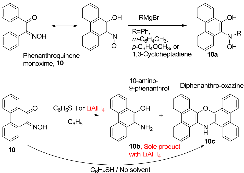
Figure 9. Reactions of Grignard reagents and reductions—Mustafa and Kamel [68].
