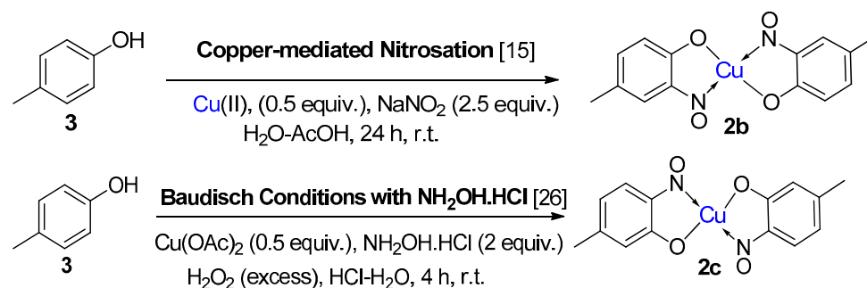
Scheme 2. A clear distinction between copper-mediated aromatic nitrosation of phenols and the Baudisch conditions is demonstrated by the reporting of a different major product from the same starting material (3) [15,26].
