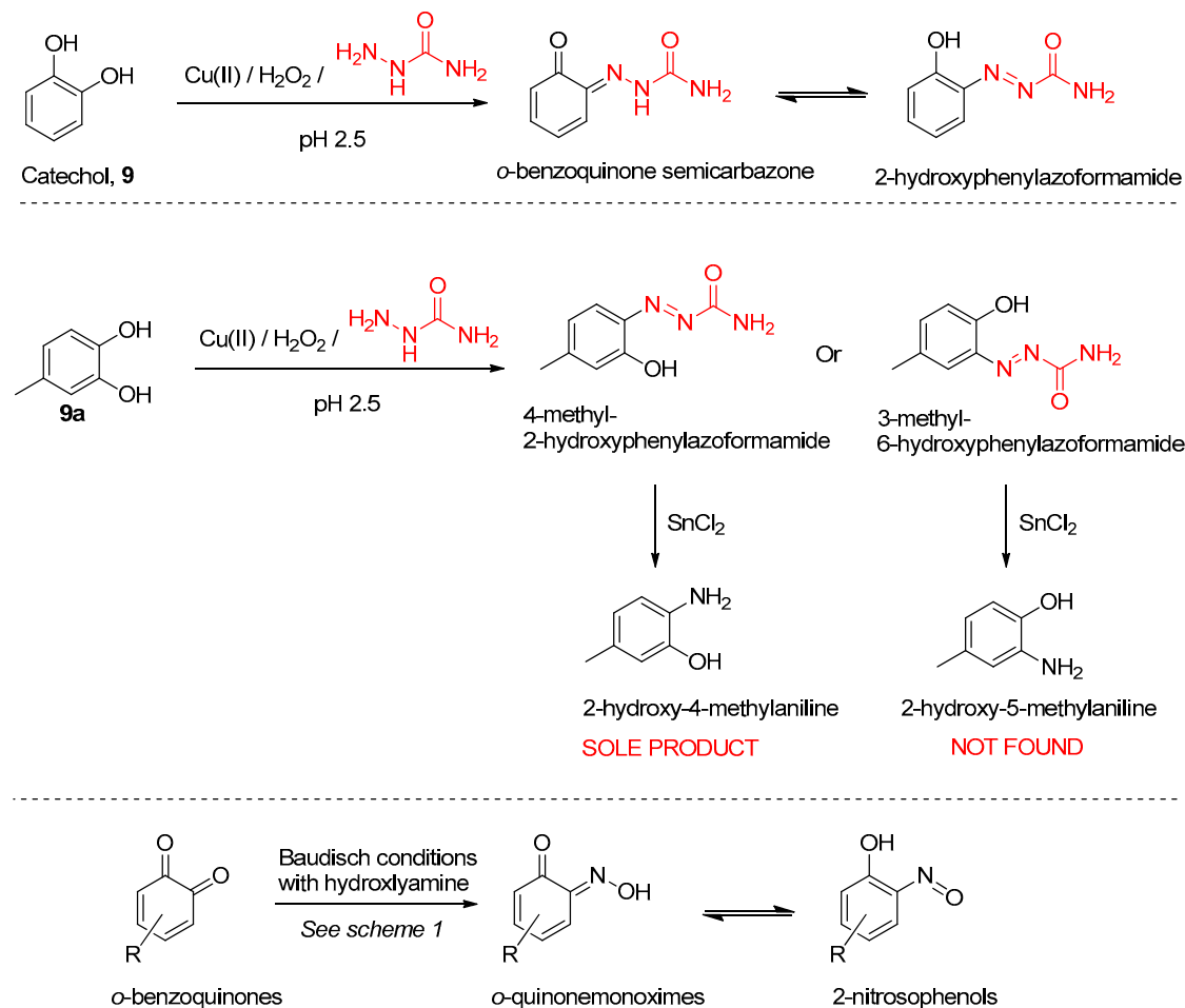
Scheme 7. Reactions from Maruyama et al. [26,42].
