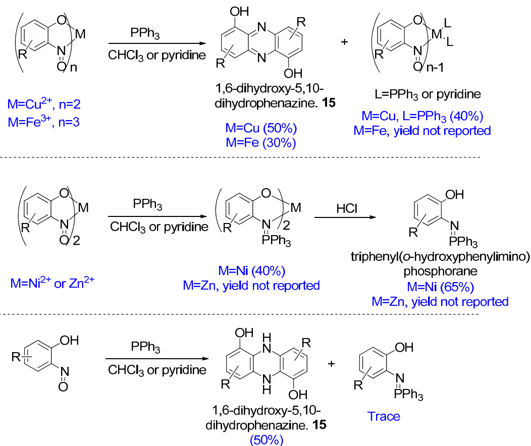
Figure 12. Reactions reported by Charalambous et al. [77].
