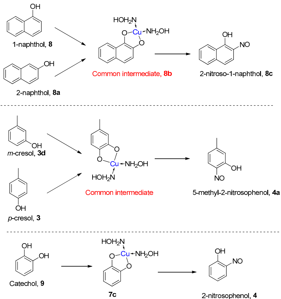
Scheme 6. Unexpected products obtained from the Baudisch reactions of naphthols, methyl-phenols and catechol, obtained by Maruyama et al. [42].
