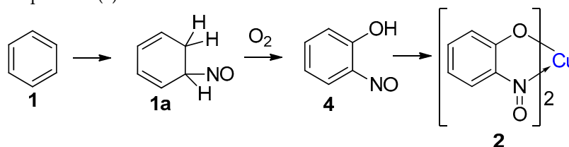
Scheme 4. The proposed sequence of copper complex formation, as suggested by Baudisch [20].
