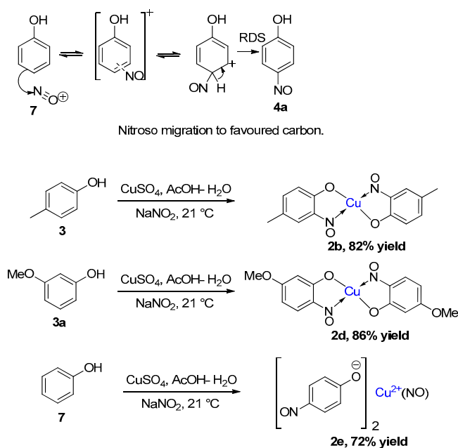
Figure 7. Accepted nitrosation mechanism for phenol in the absence of copper [33,36,63], followed by three examples of our results [41] for copper-mediated nitrosation.
