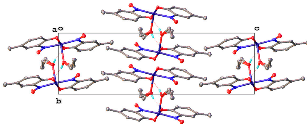
Figure 4. The unit cell of the obtained crystal structure of copper(II) bis (4-methyl-2-nitrosophenolato) with ethanol as a solvate [41,51].
