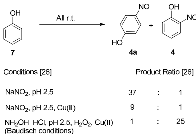
Figure 6. The results published by Maruyama [26], which appear to contradict other results from Konecny (not quantified), who instead implied that ortho -nitrosation dominated for conditions comparable to the ' \text{NaNO}_2 , pH 2.5, Cu(II)' shown [43]. The product ratios were calculated by obtaining the isolated ligand, then reacting with Cu(II) salt, separation via a preparative TLC method and finally, quantification via absorbance measurements.
