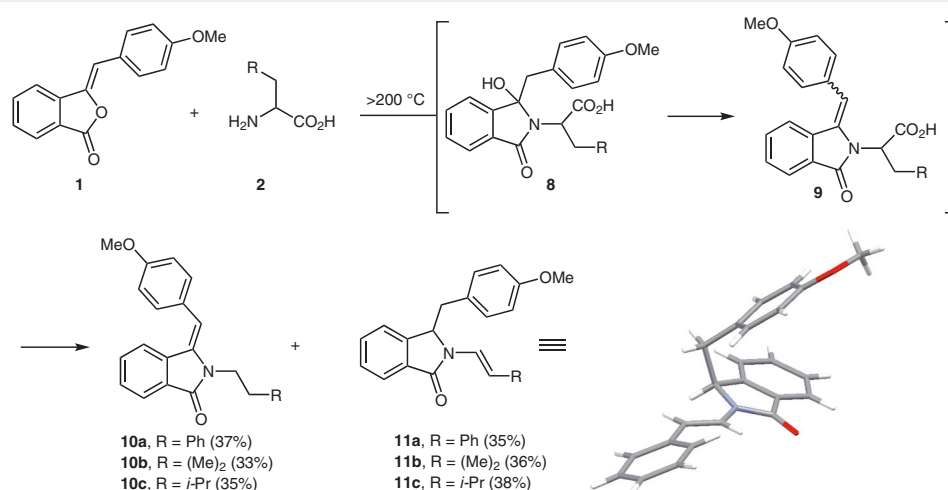
Scheme 5 Neat fusion reactions of 1 with amino acids
