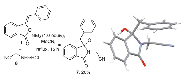
Scheme 4 Reaction of 1 with aminonitrile hydrochloride and X-ray structure of product 7
