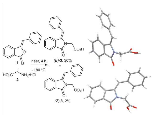
Scheme 2 Reaction with glycine giving E - and Z -configured 3 as shown by single-crystal X-ray analysis
