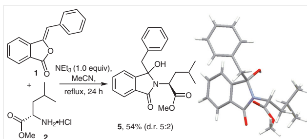
Scheme 3 Reaction of 1 with an amino ester with X-ray structure of the aminal adduct ( 5a )
