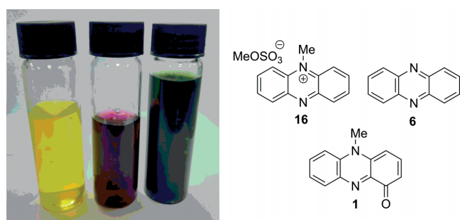
Figure 2. Photochemical colour change in the processing of phenazine salt 16 . (left to right) Starting material (SM), irradiated mixture 20 + 21 , product development upon basification in the presence of oxygen ( 6 + 1 ).
