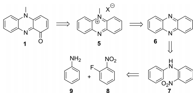
Scheme 2. Planned retrosynthesis to pyocyanin ( 1 ).
