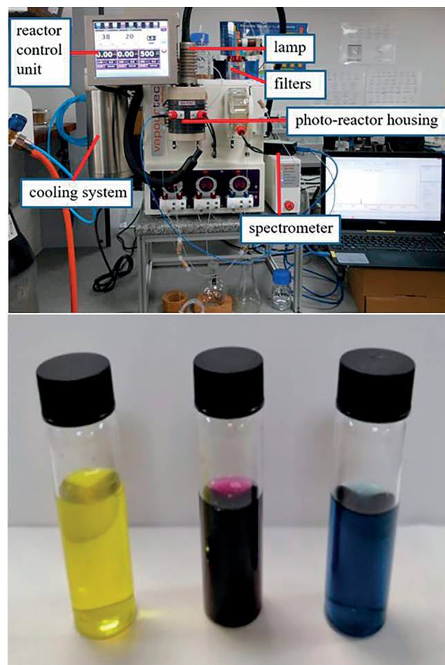
Figure 1. Flow reactor (top). Flow photochemical colour change in the processing of phenazine salt 16 (bottom). Starting material (SM), irradiated SM, product development upon basification of the red/purple sample.
