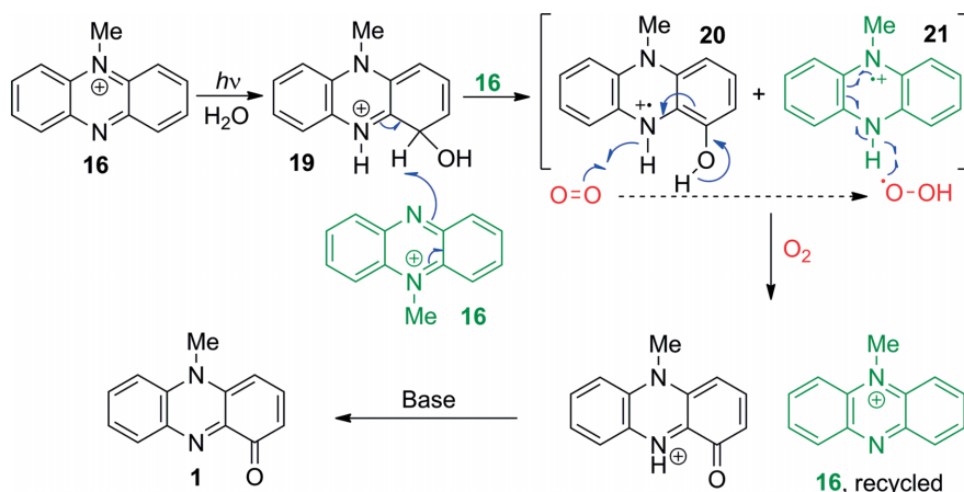
Scheme 7. Mechanism for the photosynthesis of pyocyanin (1).
