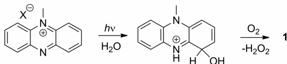
Scheme 5. Alternative synthesis proposals for formation of pyocyanin ( 1 ).
