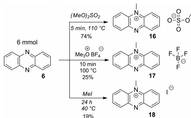
Scheme 4. Methylation to the corresponding ammonium salts 16–18 .
