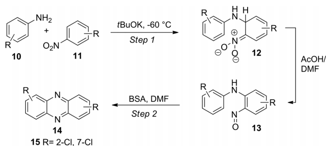
Scheme 3. Alternative general route to phenazines 14 .
